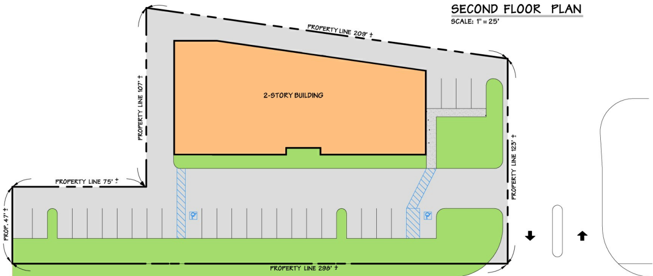
SITE PLAN SCALE: 1" = 50' 23231 LA PALMA AVENUE, YORBALINDA
